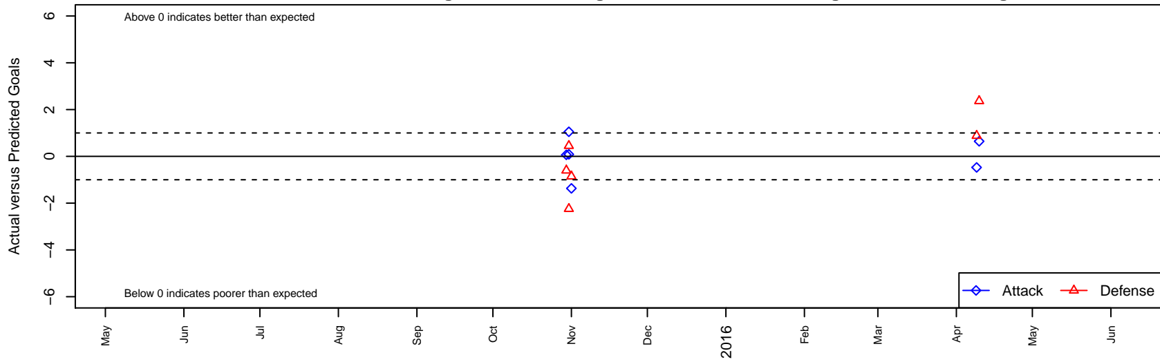
Real Colorado Edge 02 Select B01 Dots are actual minus expected GF (blue circles) and GA (red triangles). Blue line is smoothed change in attack strength. Red is smoothed change in defense strength.
